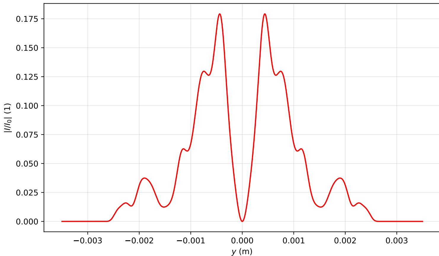
Intensity profile I(x=0, y, z=3.264)/I_0 , P_{in}=9.0P_{cr} , artificial time
